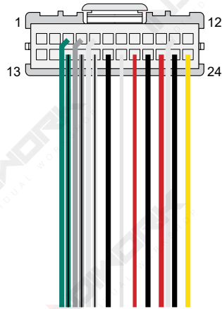
POWER / CAN CAN-GPBENZ1901-K2
